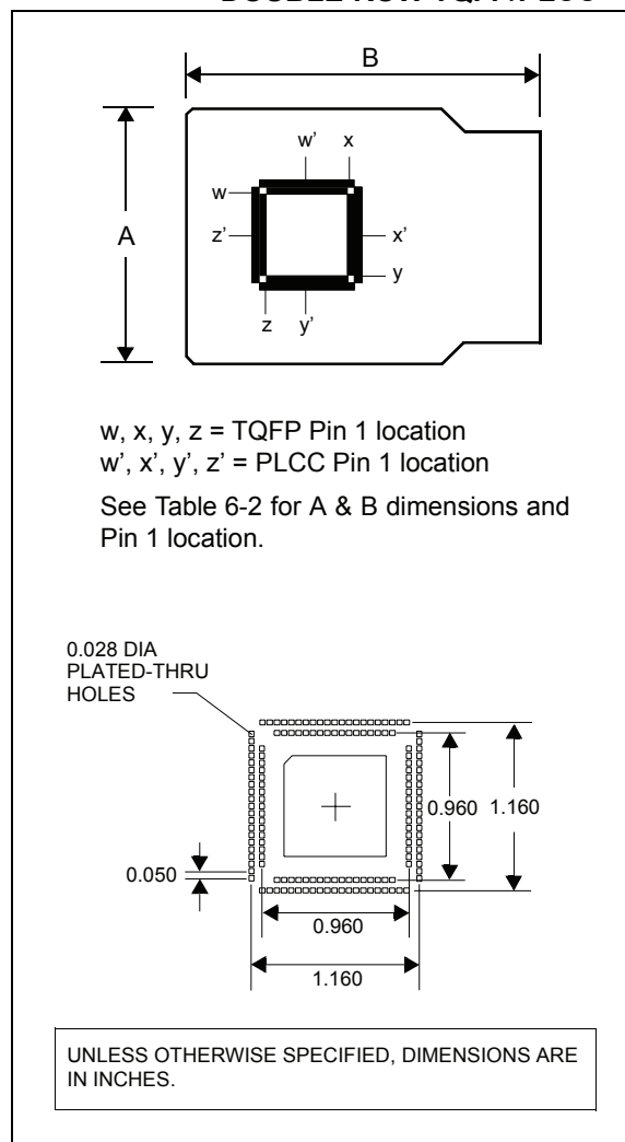
FIGURE 6-3: DVA DRAWING – DOUBLE-ROW TQFP/PLCC
