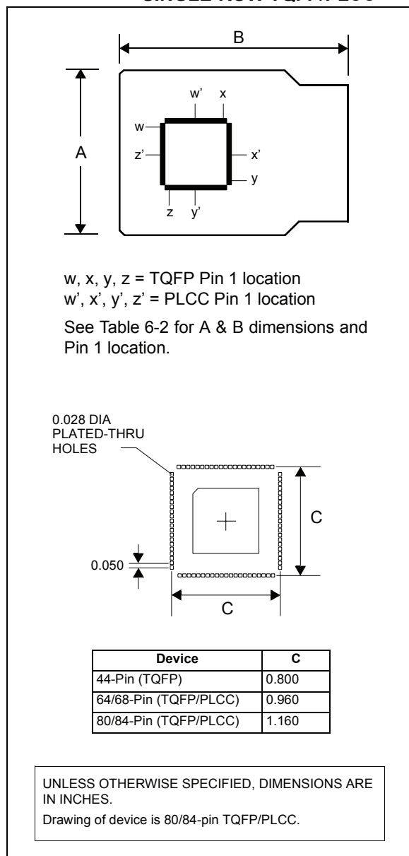
FIGURE 6-2: DVA DRAWING – SINGLE-ROW TQFP/PLCC
